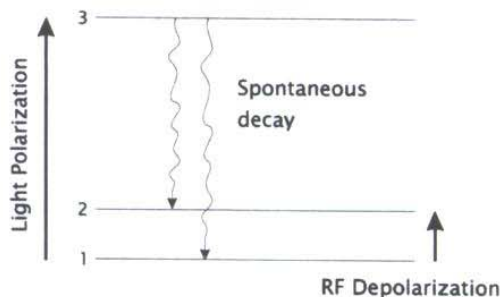
Figure 2 Quantum mechanics of alkali vapour system.
