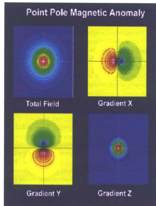
Figure 5 Comparison of total field and gradient results for the same target. (From Hogg et al., 2004)
