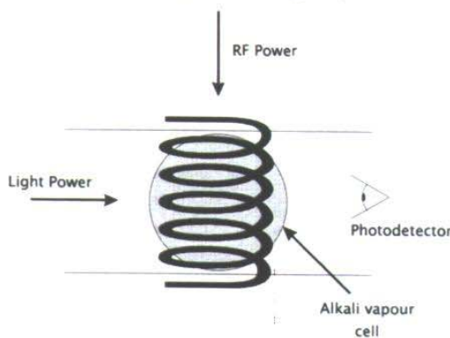
Figure 1 Generic alkali-vapour magnetometer.
